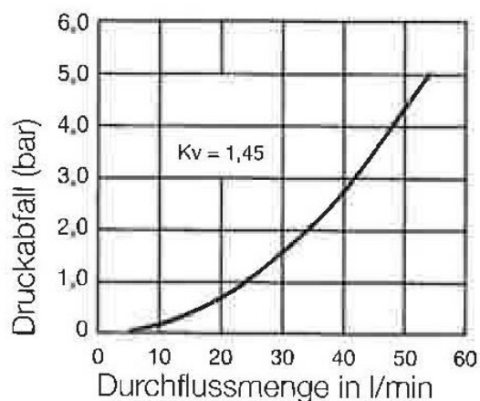
246.13 – G 3/8
